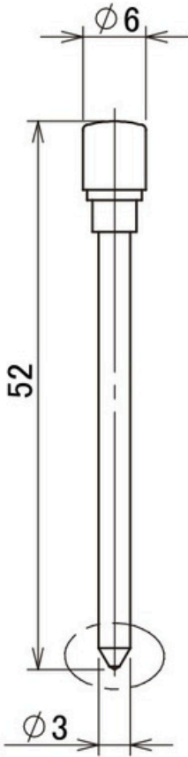
Standard Pin
